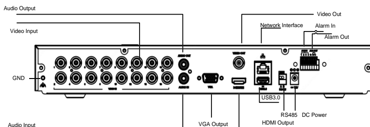
Rear View of HNRXAI16
